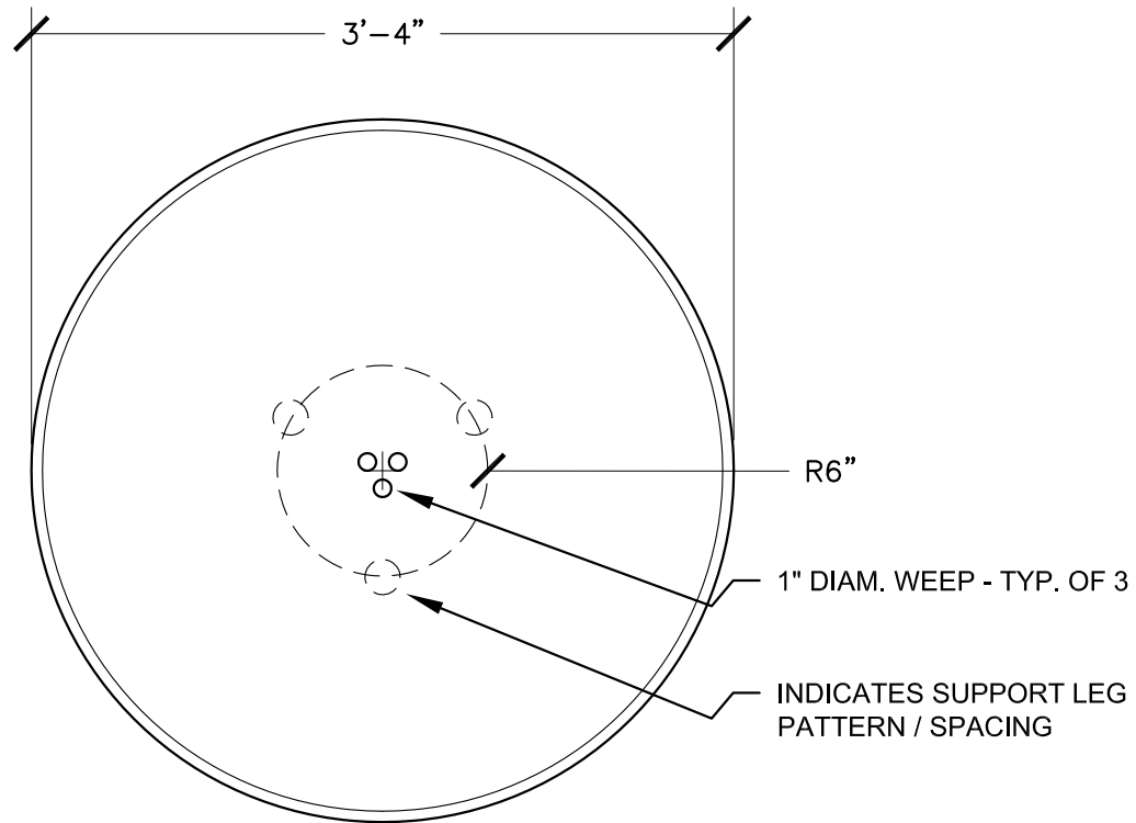
PLAN VIEW
