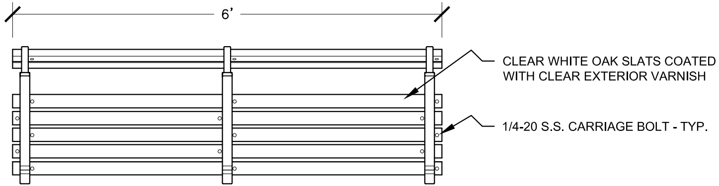
PLAN VIEW
