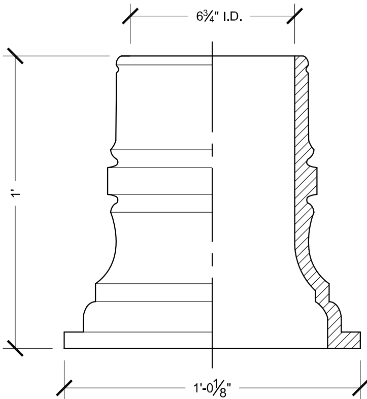
ELEVATION / SECTION
