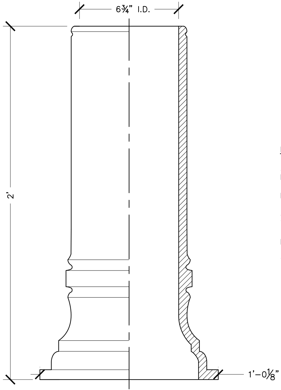
ELEVATION / SECTION
