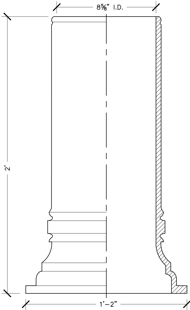
ELEVATION / SECTION
